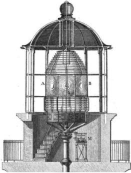
Sketch of a 1st order Fresnel lens in a watch room.
