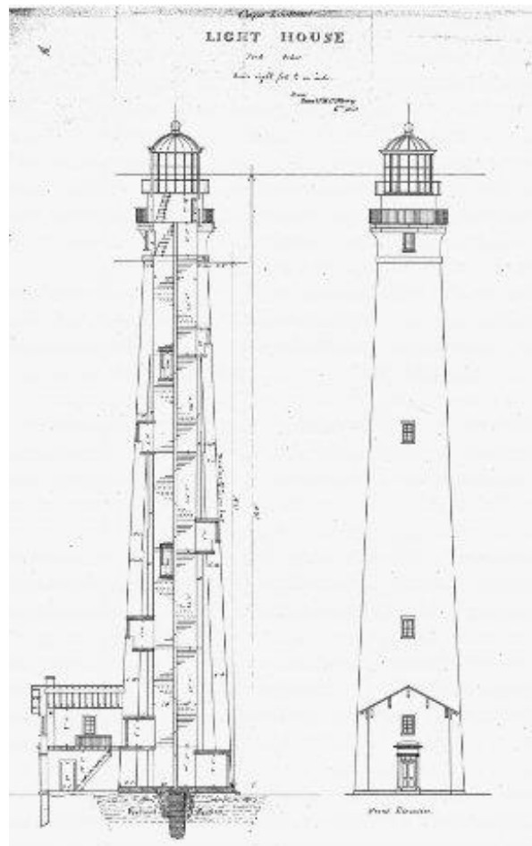
Architectural Plan for 1859 Lighthouse The attached house shown on this architectural plan for 1859 lighthouse was not built.
